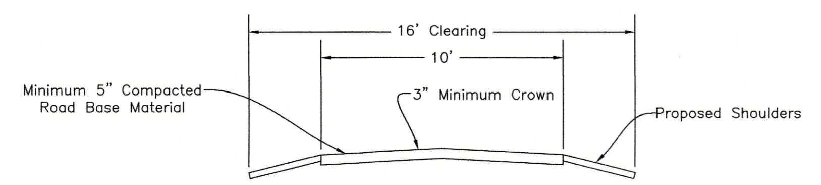
TYPICAL CROSS SECTION Scale 1" = 4'
